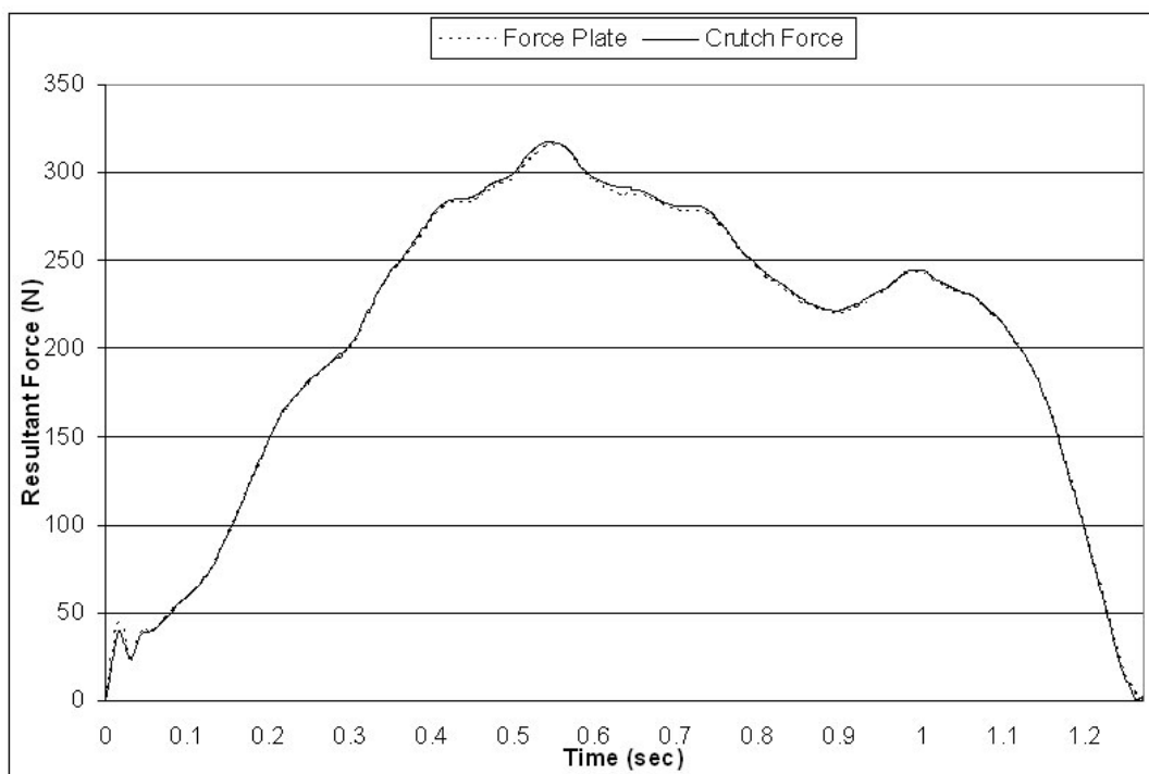
Figure 4. Resultant crutch (solid line) and forceplate (dashed line) forces simultaneously recorded.
